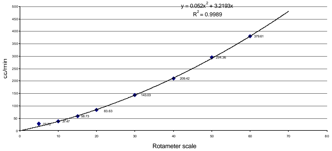
Appendix D.1 Rotameter calibration curve at 10 psig.
