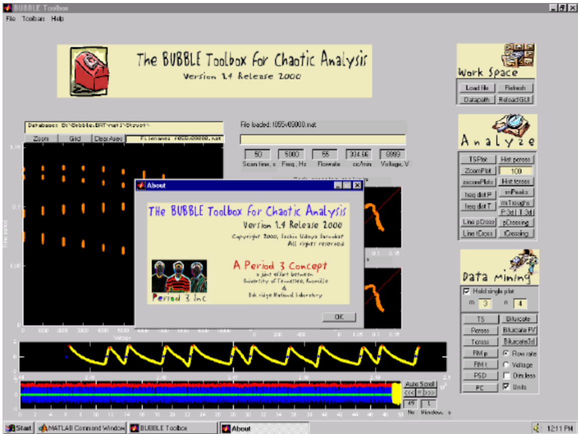
Appendix B.1 Screen shot of the BUBBLE Toolbox for Chaotic Analysis (Sarinbat, 2000).
